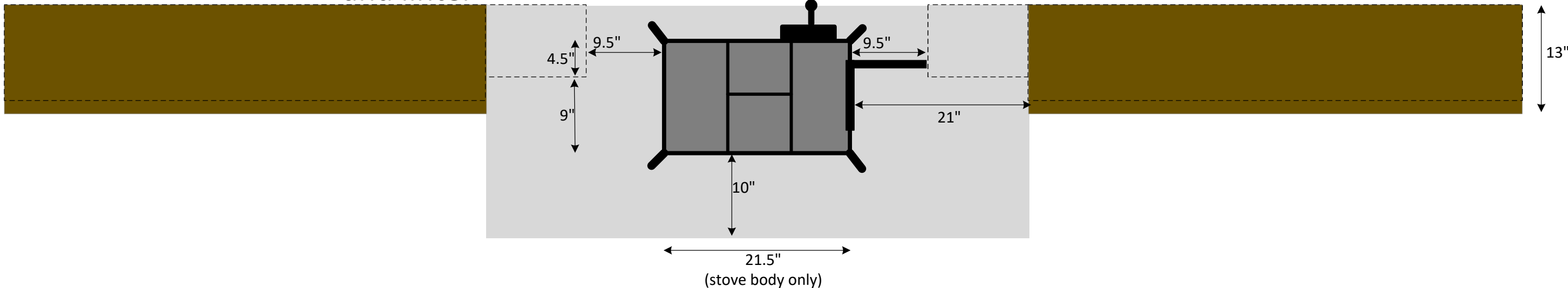
Top View w/o upper masonry and lintel
