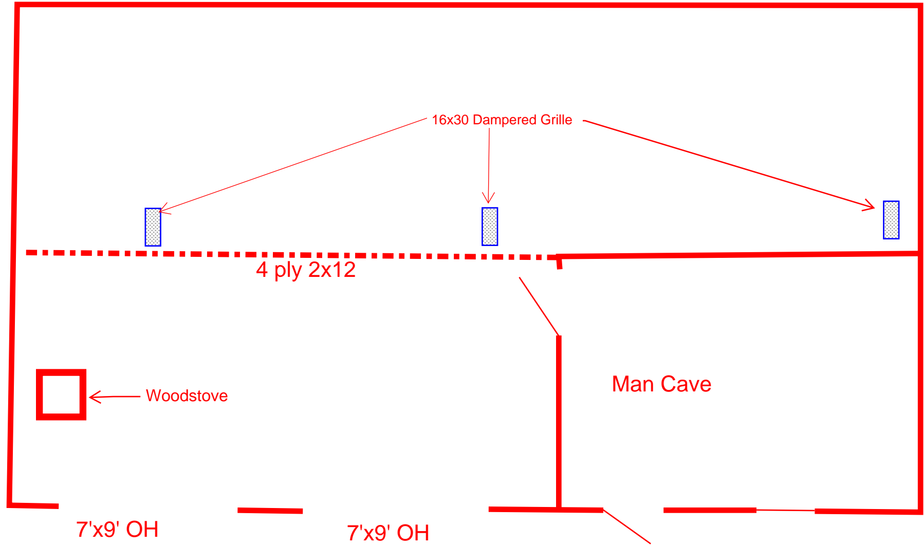
Basement Plan
