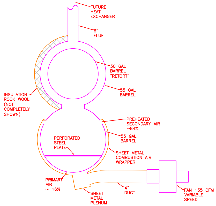
BARREL STOVE HEATER LILE 2014-08-16 NO SCALE
