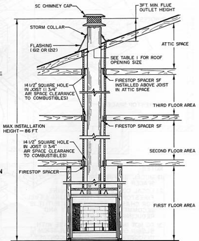
MULTIPLE STORY INSTALLATION FIGURE 10
