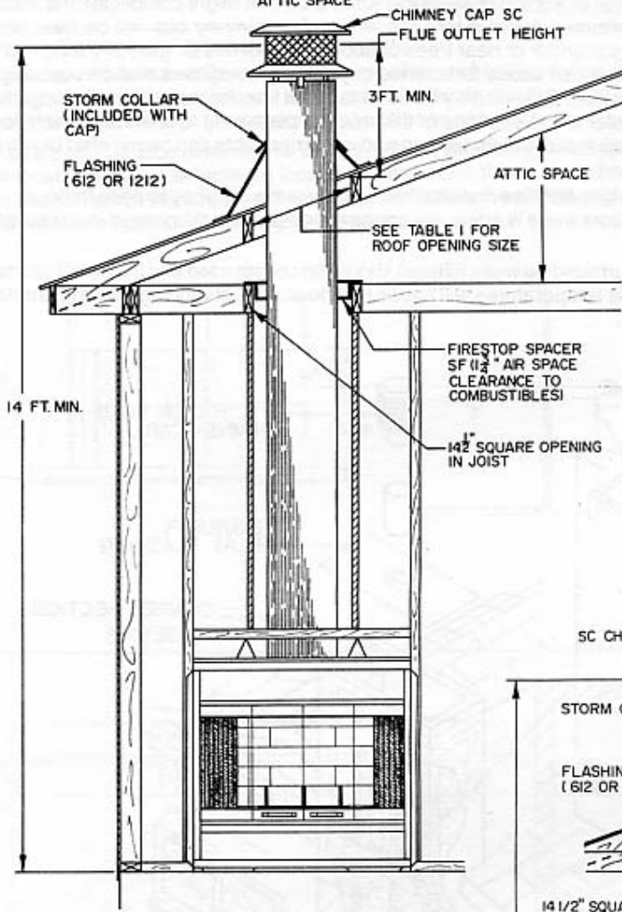
FIGURE 9 SINGLE STORY INSTALLATION WITH ATTIC SPACE
