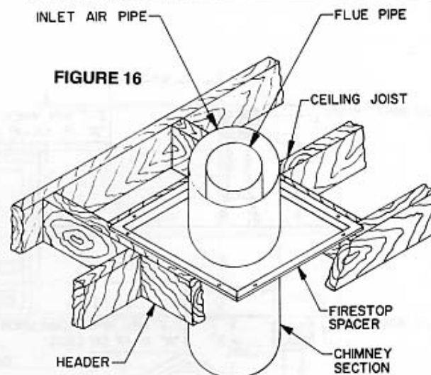
INSTALLATION OF FIRESTOP-SPACER AT FLOOR LEVELS
