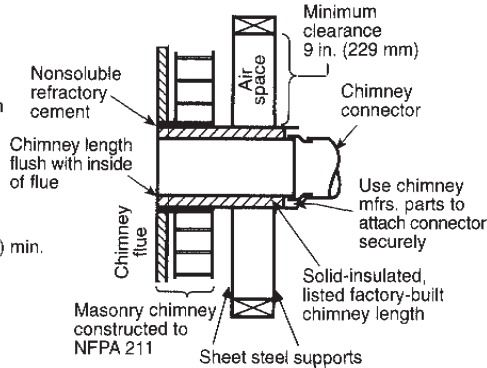
Minimum chimney clearance from masonry to sheet steel supports and combustibles 2 in. (51 mm)
