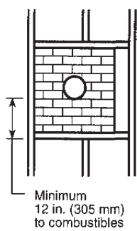
Masonry chimney constructed to NFPA 211
