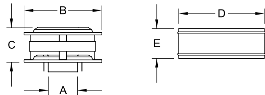
Vertical rain cap (PCR) with rain/wind shield (PRCW)
