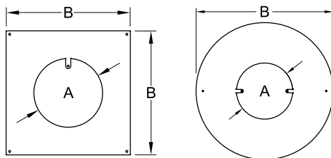
Trim plate (TP)
