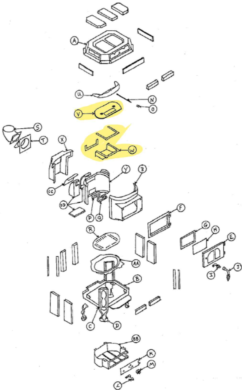
HEARTHSTONE III EXPLODED VIEW
