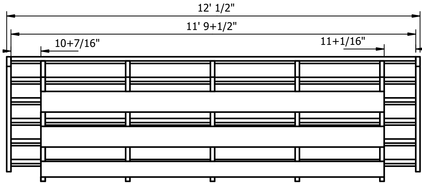
Front View
