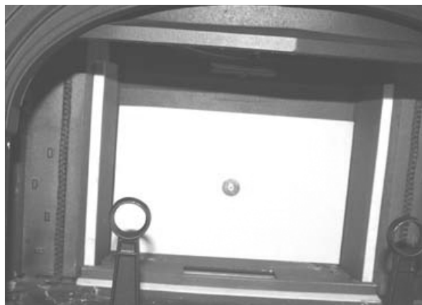
Insulator Board - 30005269 bolted to back
