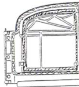
Right Door: Door to Front - 3' of 7000910 - 7/16" Round Black Gasket; Glass Seal - 3½' of 1203556 - 3/16" 4ND Black Gasket
