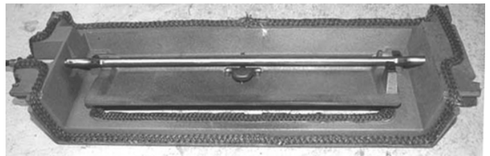
Damper Housing: Housing Seal - 6' of 30001910 - 7/16" Adhesive Gasket; Damper Opening - 3½' of 1203588 - 5/16" Medium Density 6ND
