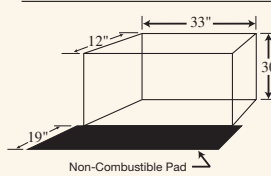
Recommended Framing Dimensions Zero Clearance Units
