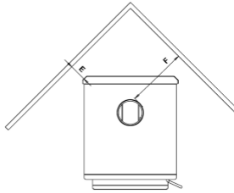
Corner Installation
