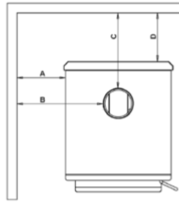
Parallel Wall Installation
