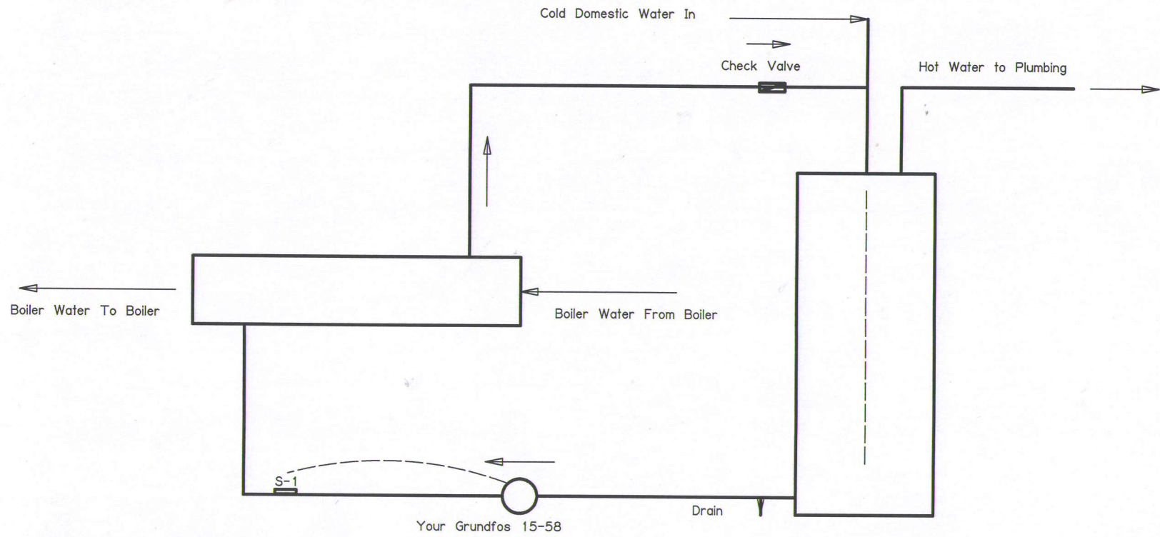
S-1 Pump Control
