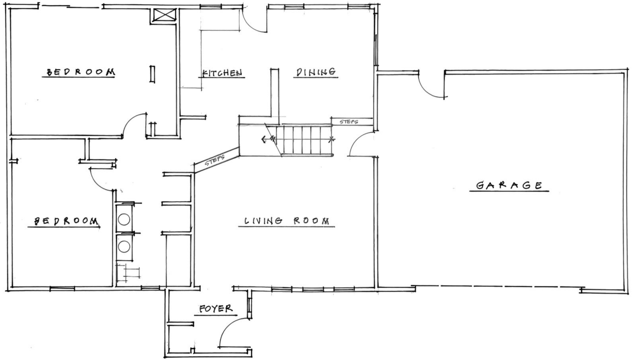
FLOOR PLAN 1/4" = 1'-0"
