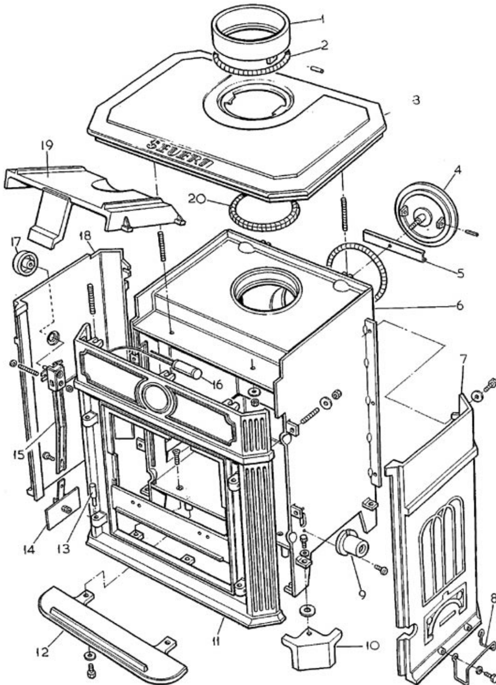
COALBROOKDALE SEVERN STOVE (BOILER) MAIN BODY ASSEMBLY
