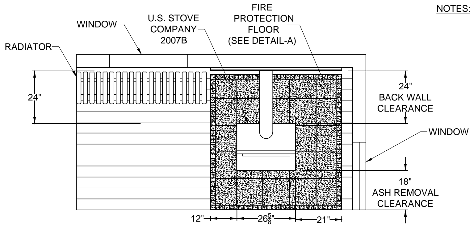
TOP VIEW SCALE 1=1
