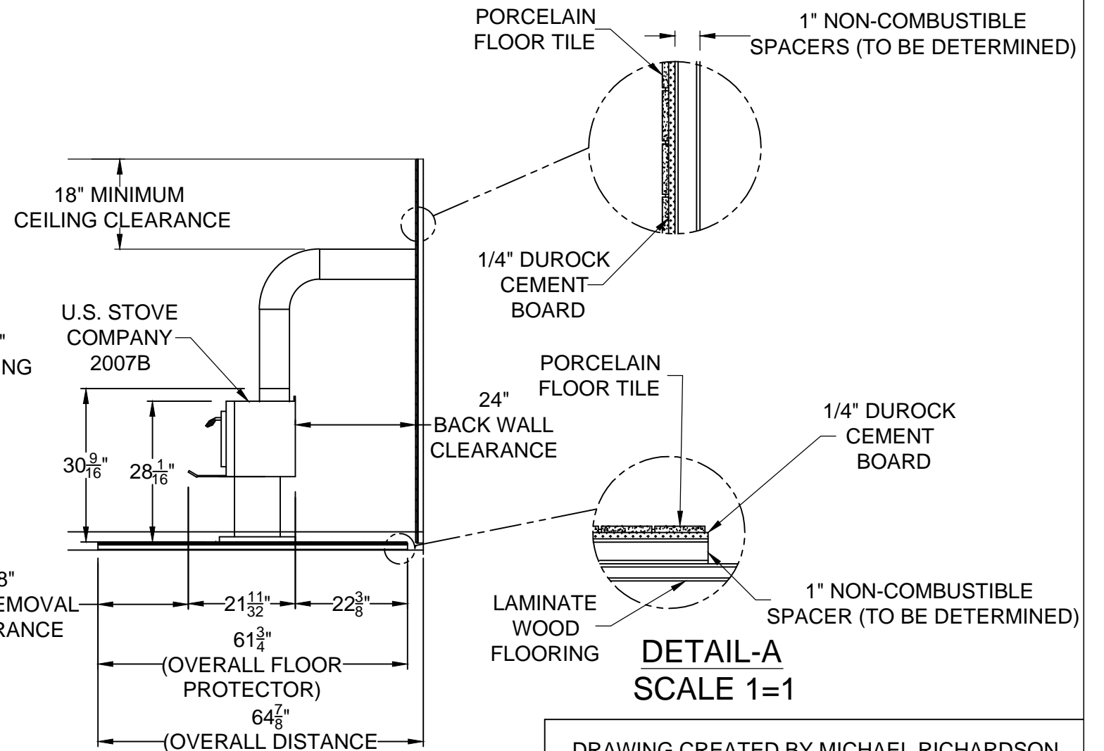
SIDE VIEW SCALE 1=1
